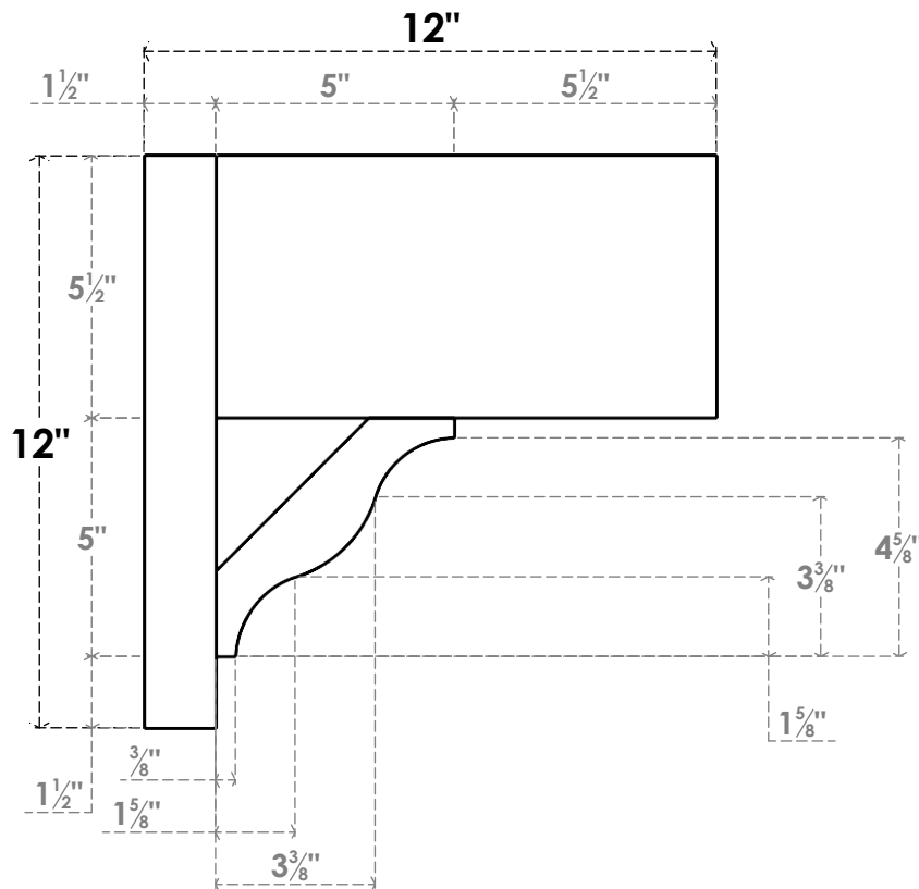
SIDE PROFILE
